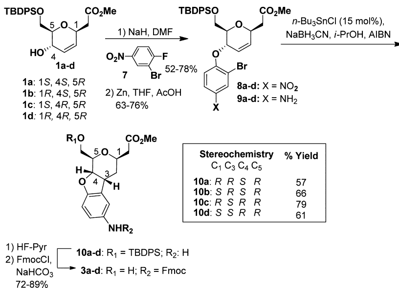
Scheme 2. Tricyclic Lactam Formation via Intramolecular S N Ar
