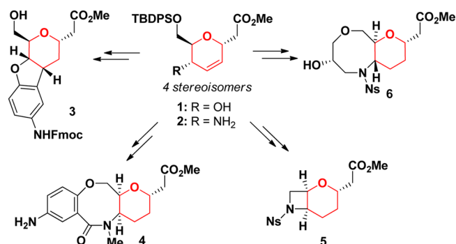
Figure 1. Synthesis of fused bi- and tricyclic ring systems from a C-glycoside template.
